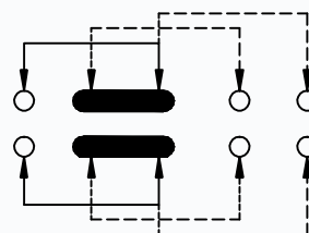
SCHEMATIC (SHORTING)
