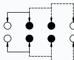
SCHEMATIC (NON-SHORTING)
