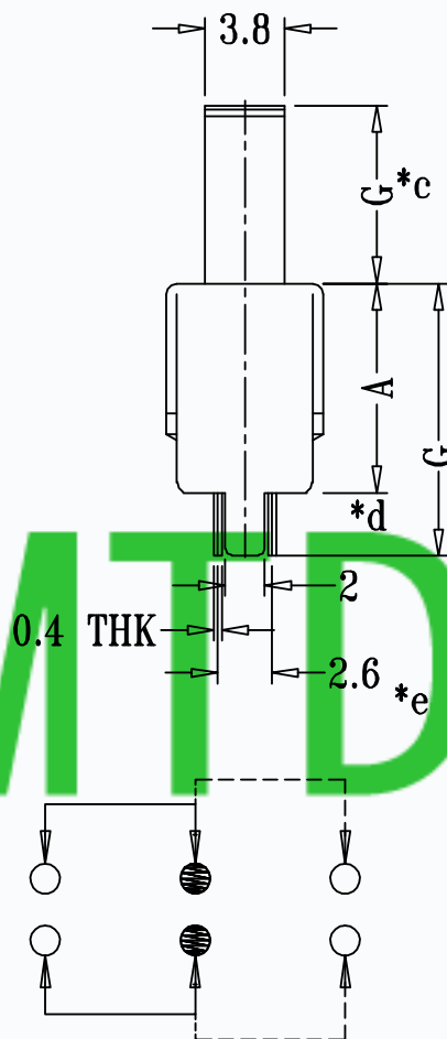
SCHEMATIC (NON-SHORTING)
