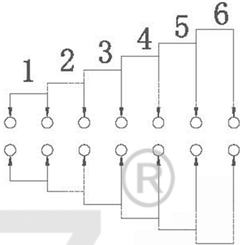
SCHEMATIC (NON-SHORTING)
