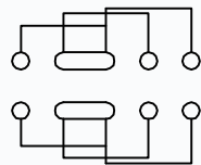
SCHEMATIC (SHORTING)
