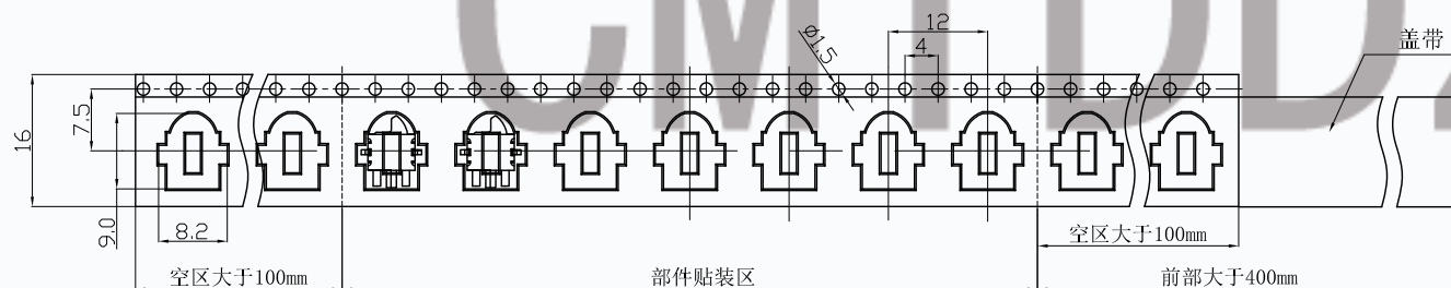
CARRIER TAPE
